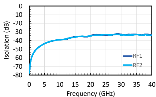
Figure 9 - Isolation (DC-40 GHz).
