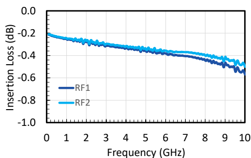
Figure 4 - Insertion Loss (DC-10 GHz).
