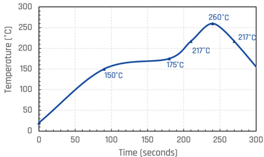
Figure 14 - Recommended Reflow Profile for the AIR40SEO soldering process.
