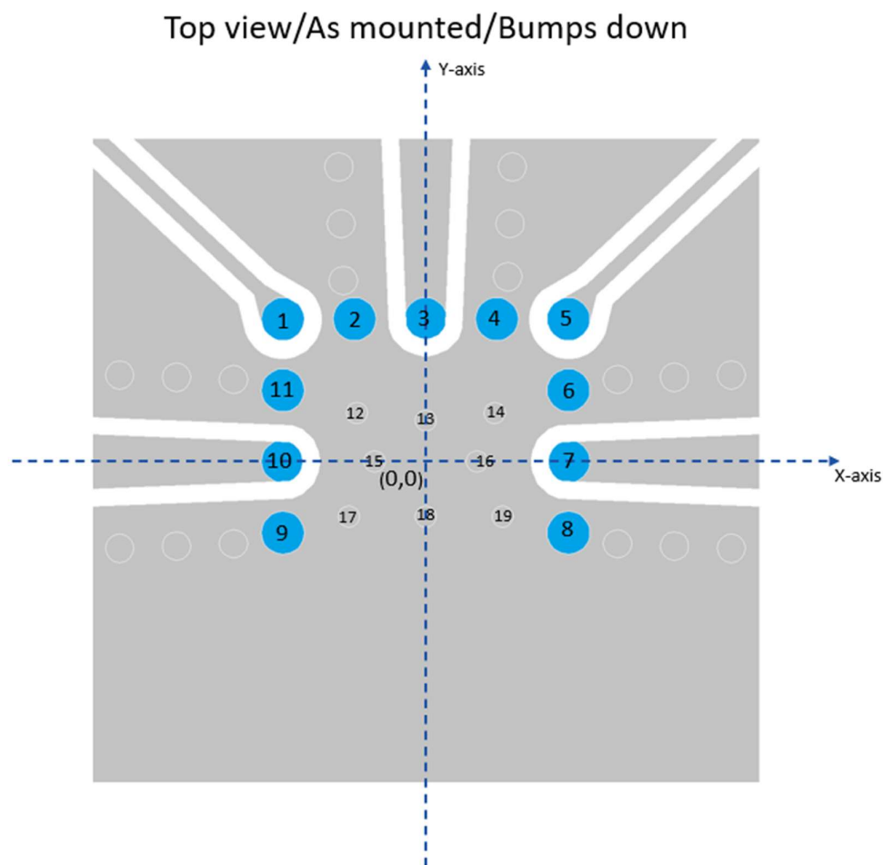
Figure 13 - Top view of the PCB.
