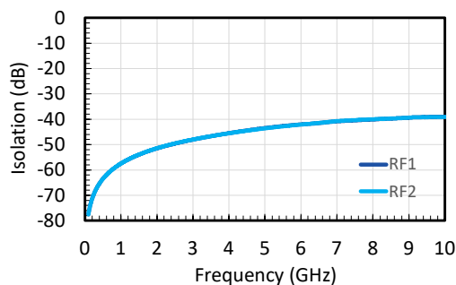
Figure 8 - Isolation (DC-10 GHz).
