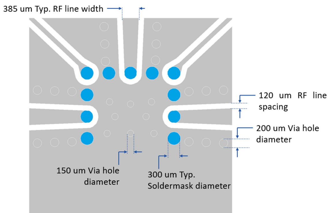
Figure 12 : Recommended PCB layout for a substrate RO4350B
