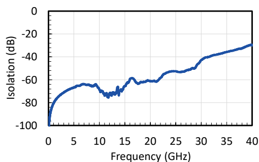
Figure 7 - Cross Talk (RF1-RF2).
