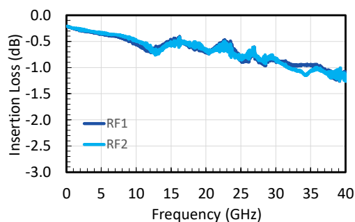
Figure 5 - Insertion Loss (DC-40 GHz).
