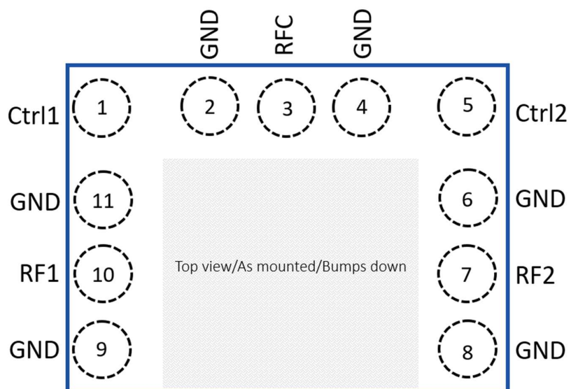
Figure 10 - AIR40SEO Pin Configuration (Top view).
