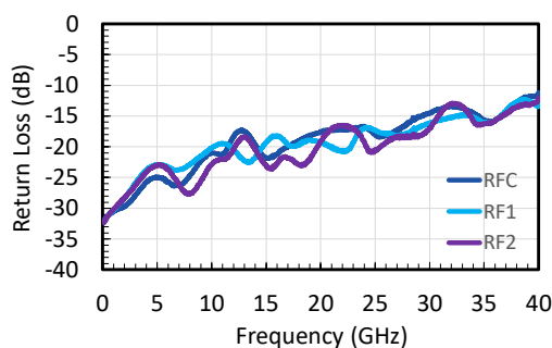
Figure 6 - Return Loss.
